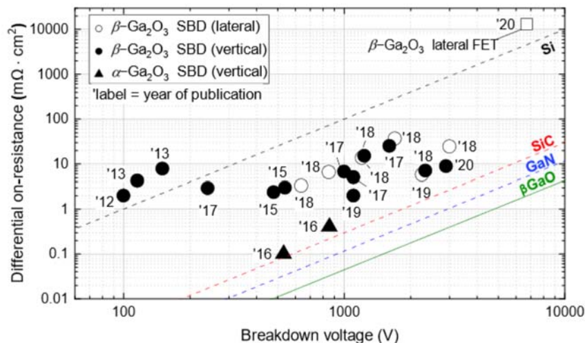
Figure 3.51: Unipolar on-resistance versus breakdown-voltage limits for important power semiconductors (lines) and exemplary achievements reported for gallium oxide devices (symbols).
