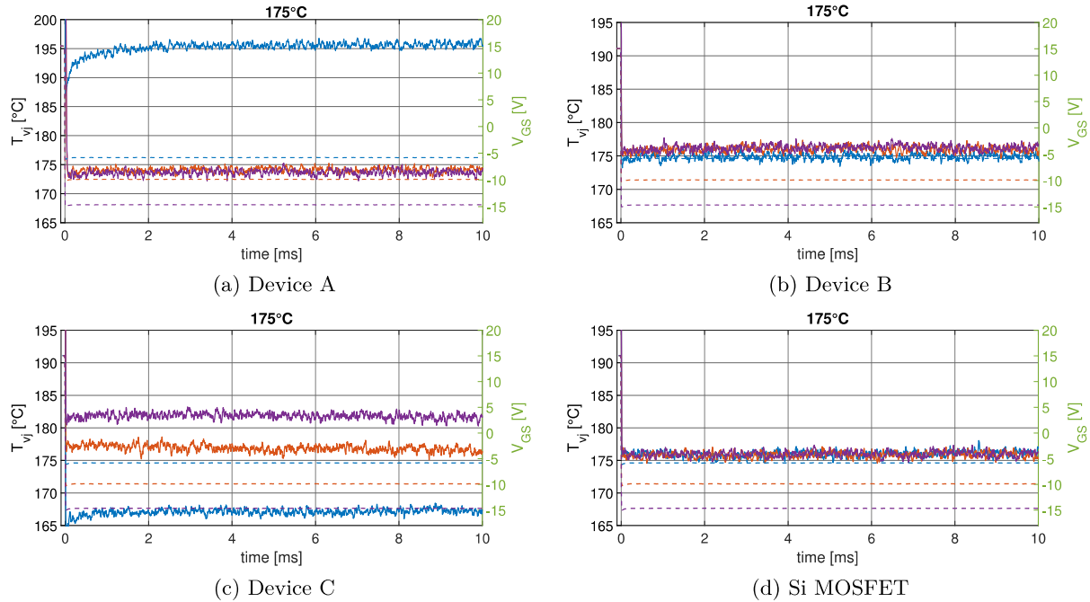
Figure 3.48: Results of the V_{SD}(T) -method applied to different commercial 1200V SiC MOSFETs and one Si MOSFET for reference at constant junction temperature of 175 °C and varying turn-off gate voltages V_{GS,off} = \{-6 \text{ V}; -10 \text{ V}; -15 \text{ V}\} ; I_{sense} = 5 \text{ mA} ; V_{GS,on} = 15 \text{ V}
