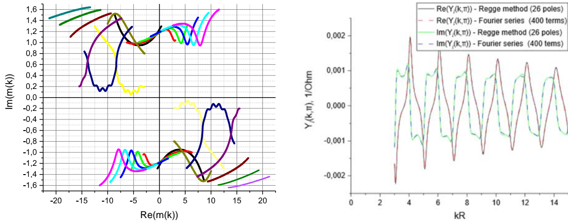
(a) Regge trajectories (26 poles) for a circular loop with R = 4 \text{ m} , r_0 = 1 \text{ cm} , 0.75 \frac{1}{\text{m}} \leq k \leq 3.875 \frac{1}{\text{m}} (b) Frequency dependence of the admittance function for current for the circular loop ( R = 4 \text{ m} , r_0 = 1 \text{ cm} ) calculated by Regge and Fourier methods. The voltage source and observation point are arranged at the points \varphi = 0 and \varphi = \pi .
