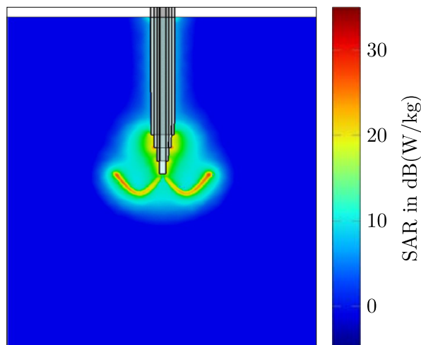
Figure 3.31: Simulations of the specific absorption rate (SAR) with the aid of a bipolar umbrella electrode inside a homogeneous liver phantom at 123 MHz
