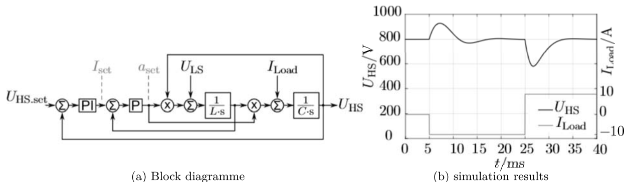
Figure 3.53: Control loop
