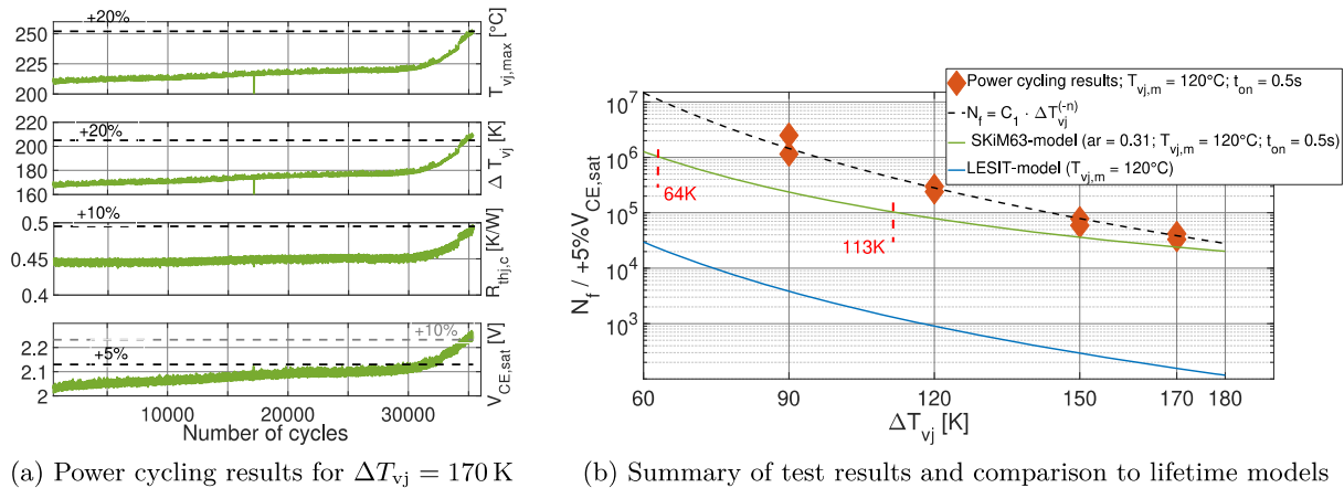
Figure 3.49: Power cycling results for T_{vj,m} = 120\text{ °C} , t_{on} = 0.5\text{ s} , t_{off} = 1.5\text{ s} ; derived Coffin-Manson model: C_1 = 2 \times 10^{17} ; n = 5.7
