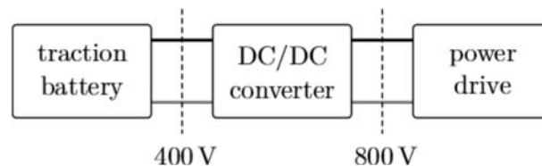
Figure 3.52: Block diagramme of the power train structure
