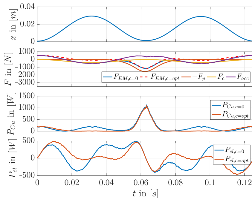
Figure 3.6: Force and power balance over a four stroke cycle with and without spring
