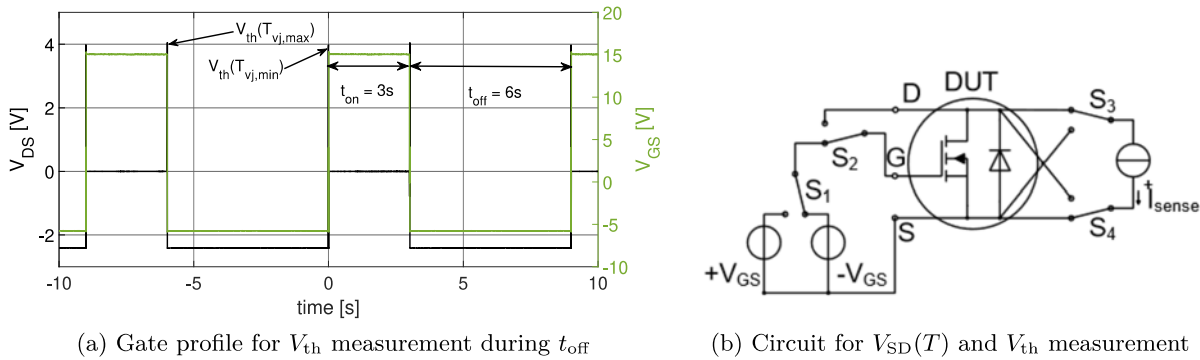
Figure 3.47: Exemplary gate profile and simplified circuit developed for combined V_{\text{SD}}(T) and V_{\text{th}} sensing
