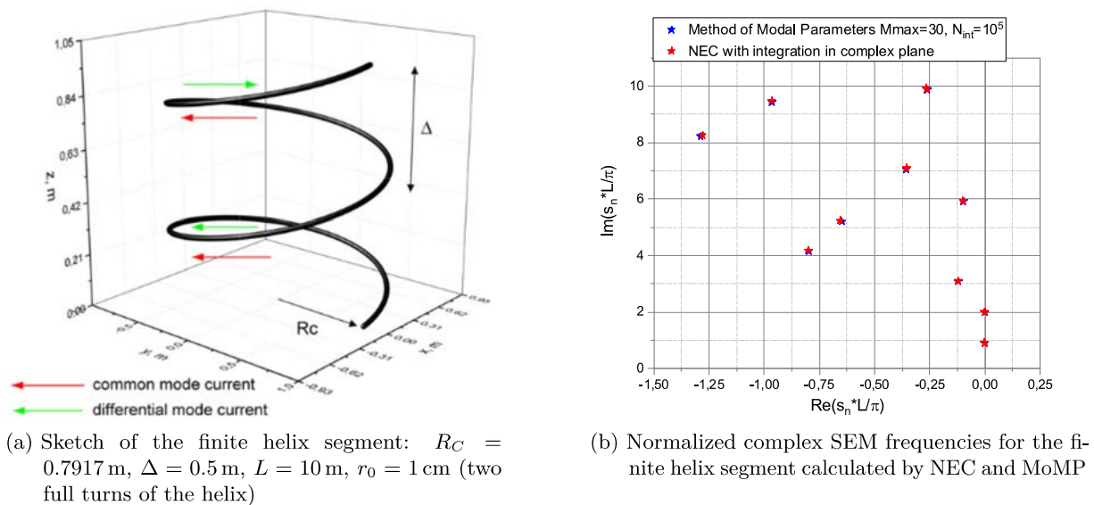
Figure 3.39: Method of modal parameters for the thin-wire open-circuit wiring structures and the singularity expansion method
